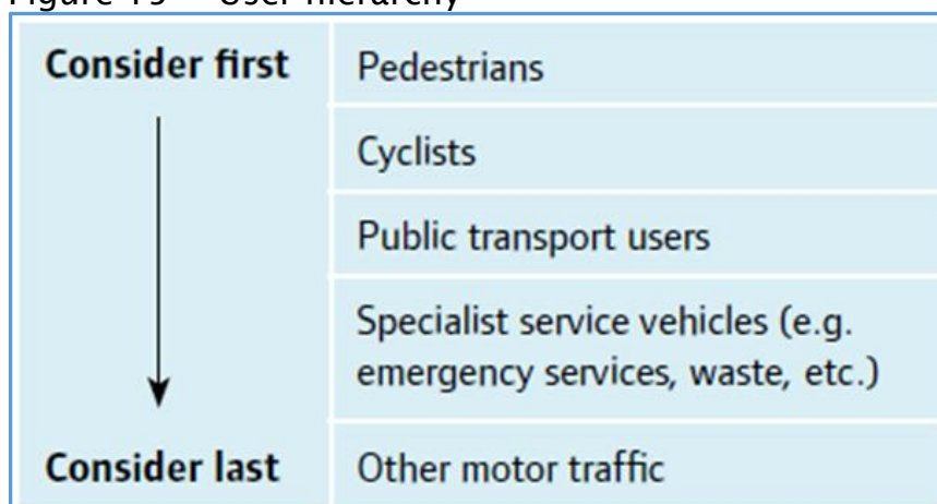
Figure 15 User hierarchy
