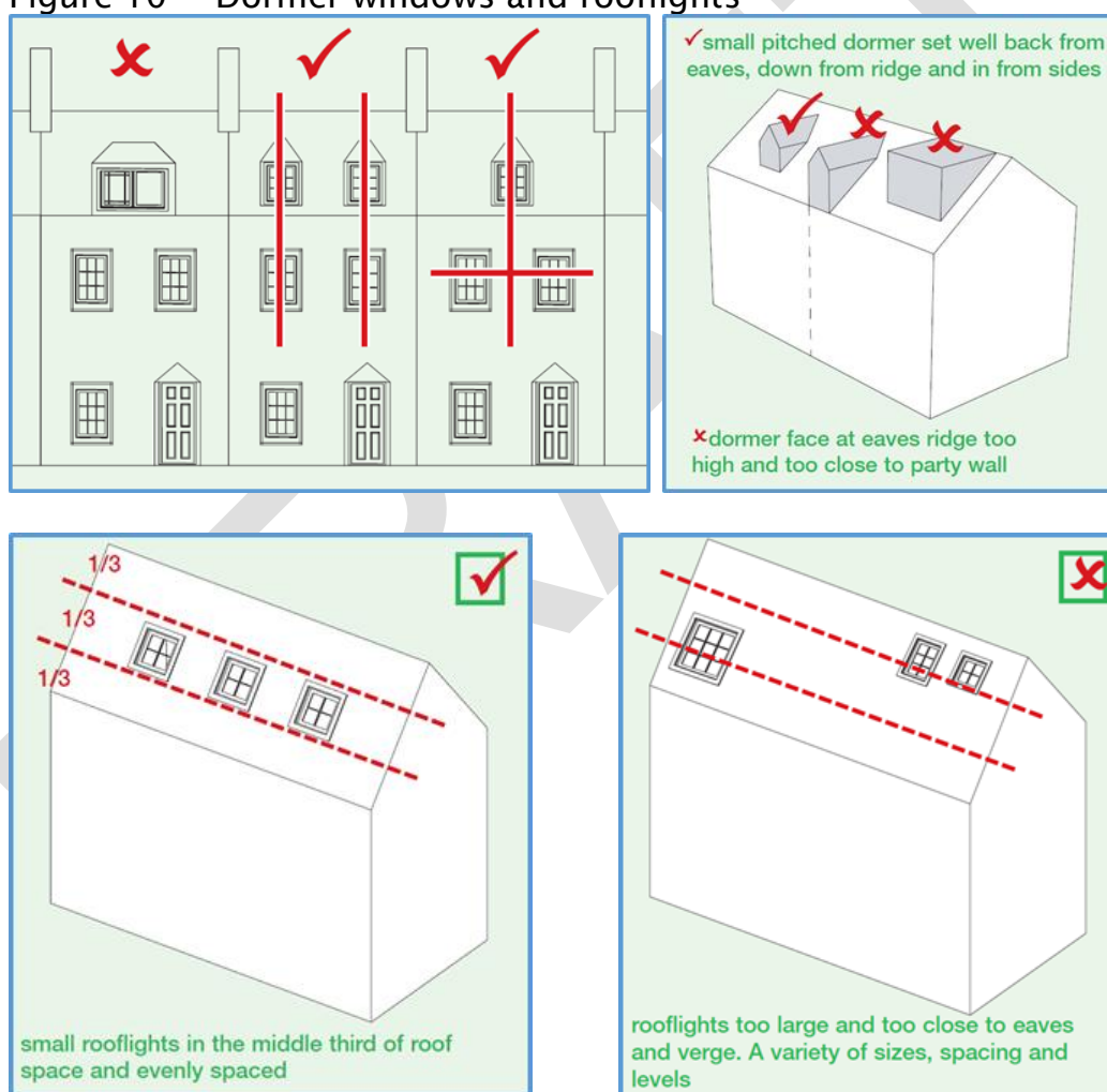
Figure 10 Dormer windows and rooflights
